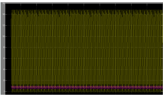
Fig.10 Thyristor Output Voltage and Current at \theta=90
